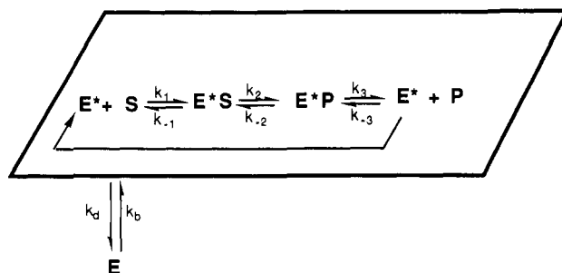
FIGURE 1: Scheme to accommodate key features of interfacial catalysis by PLA2. The species (E*, enzyme; S, substrate; P, products) shown in the box plane are in or bound to the interface, and the enzyme in the aqueous phase is shown as E. During steady-state catalysis in the scooting mode, the E to E* equilibrium is essentially completely in favor of the bound form. For a complete analysis of this formalism see Berg et al. (1991).
