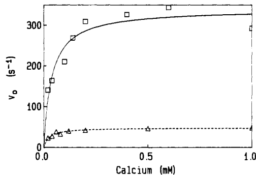
FIGURE 3: Dependence of the initial rate of hydrolysis of (squares) monothio- and (triangles) dithio-DDPM by porcine pancreatic PLA2 as a function of the calcium concentration. Reaction conditions as given in the legend to Figure 2.
